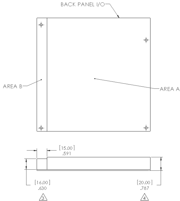
Figure 6. Thin Mini-ITX Maximum Component Height Restrictions
