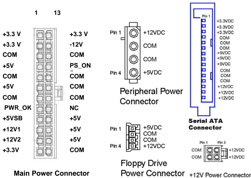
Figure 15. TFX12V Connectors (Pin-side view, not to scale)
