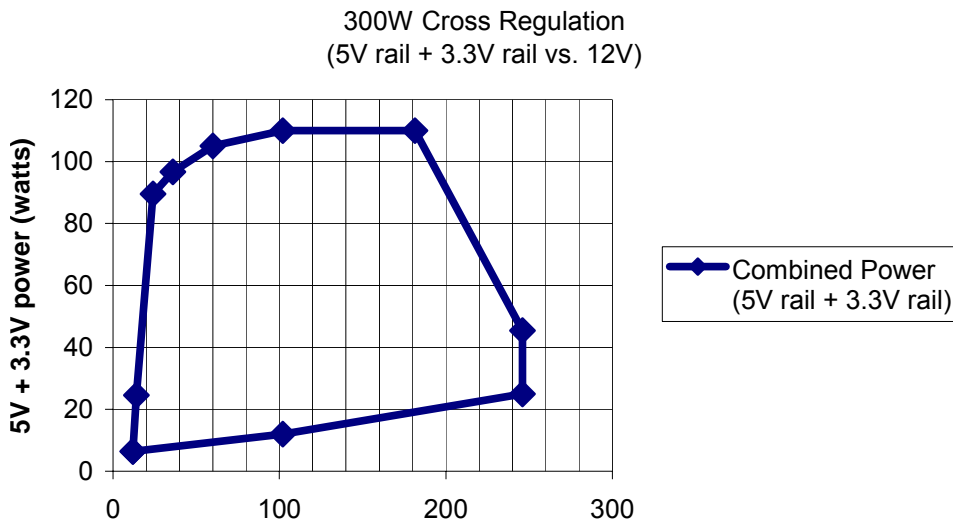
Figure 6 Cross Loading Graph for 300W Configuration Efficiency General
