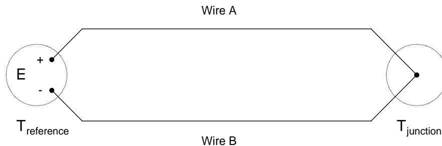
Figure 5.10: A Simple Thermocouple
